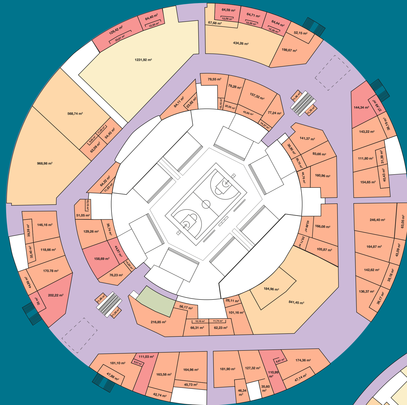
PIANO TERRA/ GROUND FLOOR
